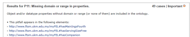
Fig. 6. An excerpt from the first important pitfall.
