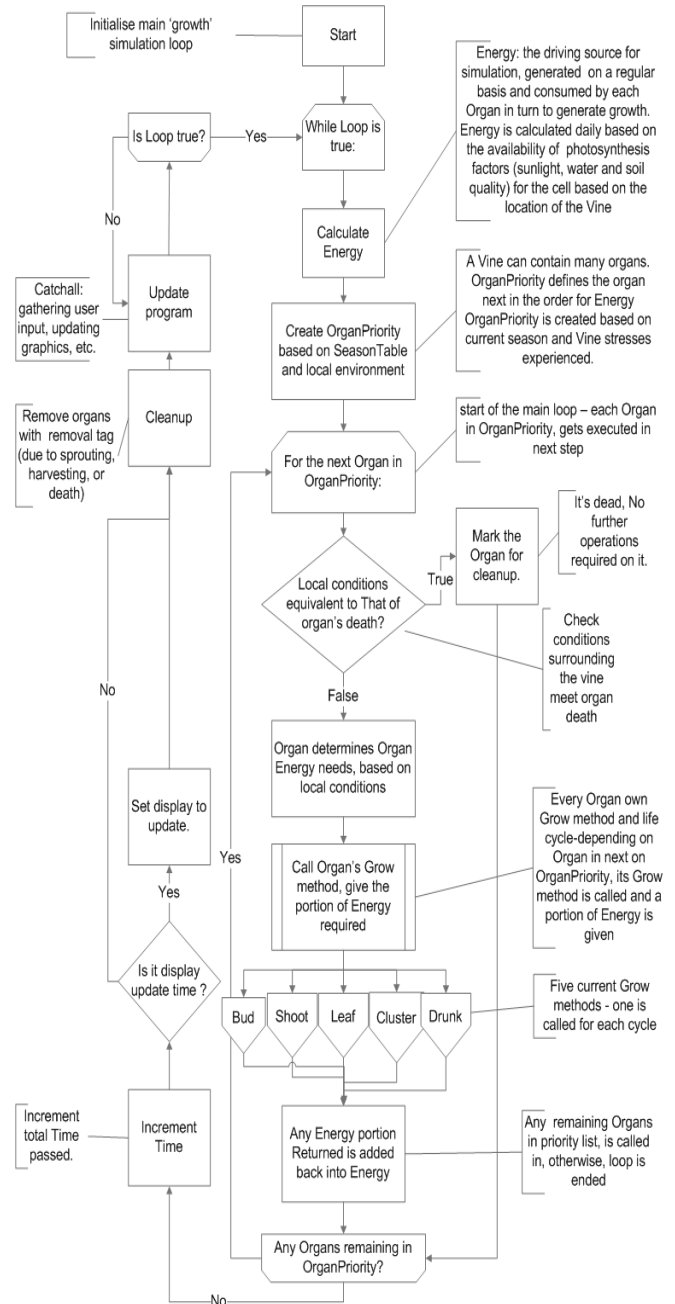
Figure 1. Schematic representation of the main processes relating to vine CA cycle. Each vine growth is displayed by a l \times l lattice simulated by vine rules.
