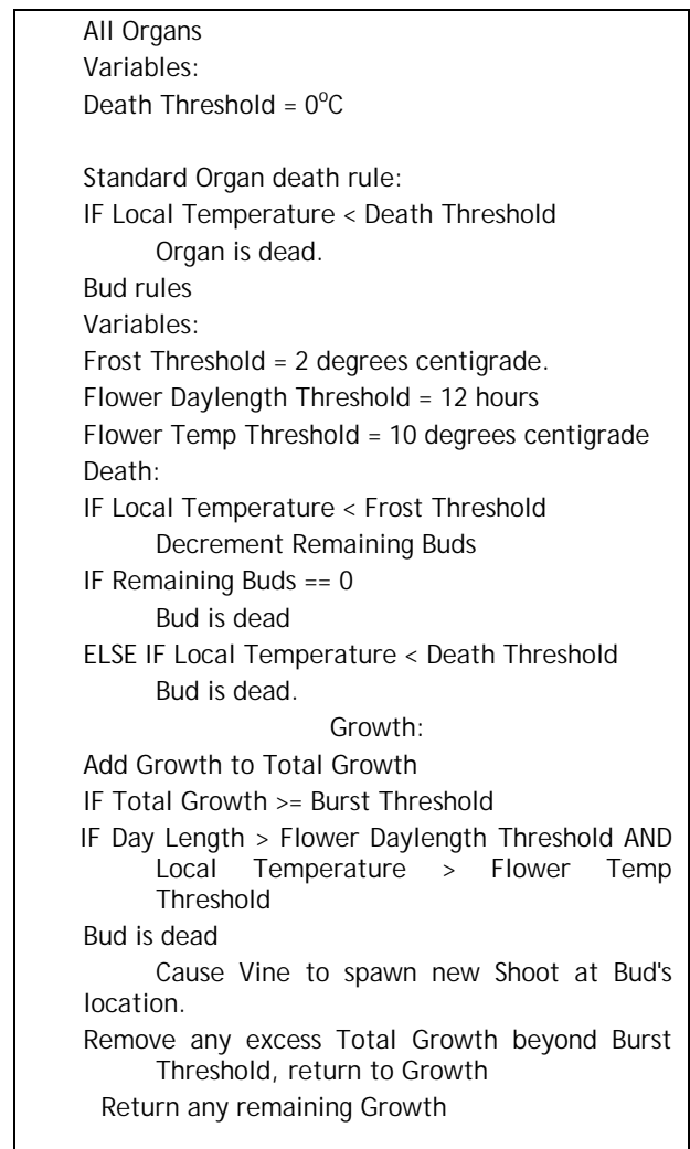
Figure 3. Field CA rules for budburst, death and growth
